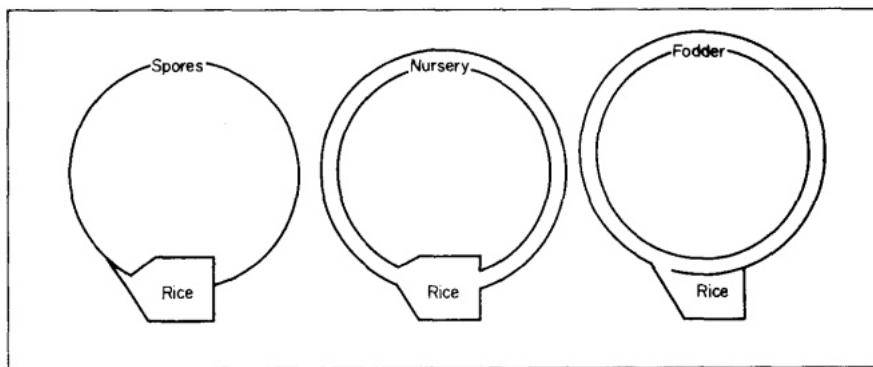
1. The three basic methods of maintaining Azolla planting material during off-seasons. These methods can be combined. About 3 wk must be allowed for germination of spores and development to dividing plants.
