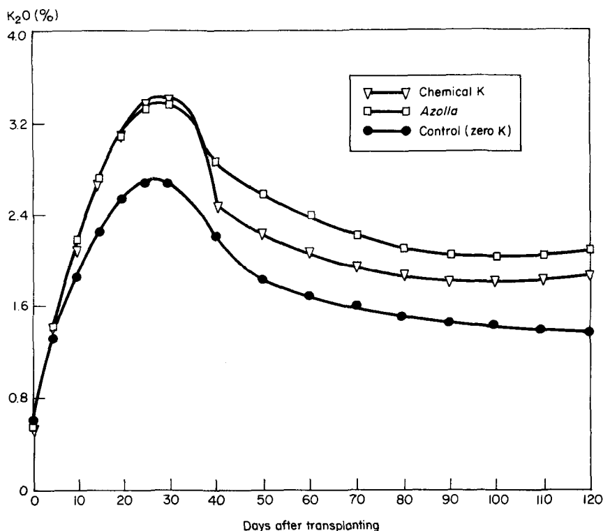
3. The dynamic change of K content in rice plant as affected by various K sources.
