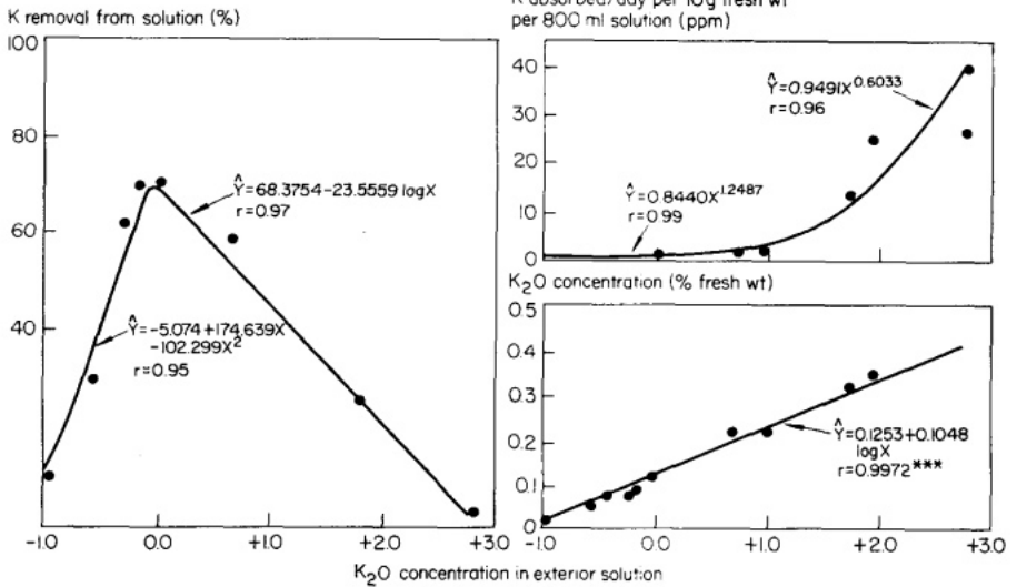
1. K absorption by Azolla from solution and K_2O content in Azolla as related to K_2O concentration in exterior water.
