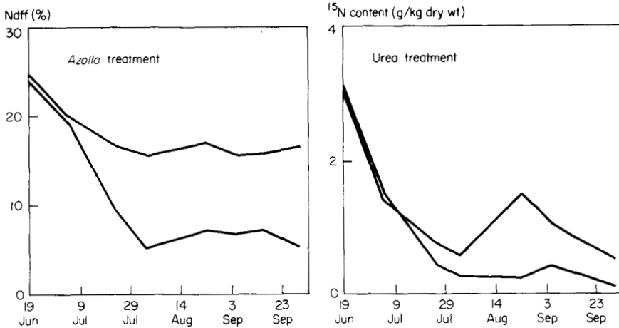
5. % Ndff and 15 N content in Azolla treatment and in urea treatment. Incorporation date for Azolla : 14 May.
