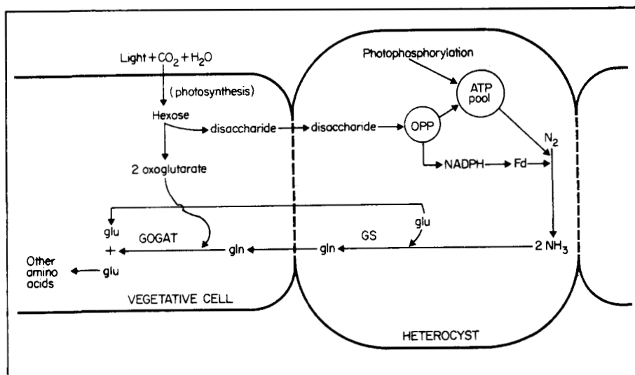
3. N_2 fixation and NH_3 assimilation pathways in vegetative cell and heterocyst.
